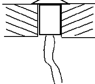
Removed Pre-wire Plug 3/8" Switch set-up inside
