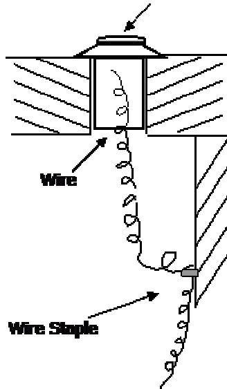
Pre-wire Plug w/Cover
